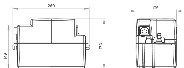
Dimensions (mm)
