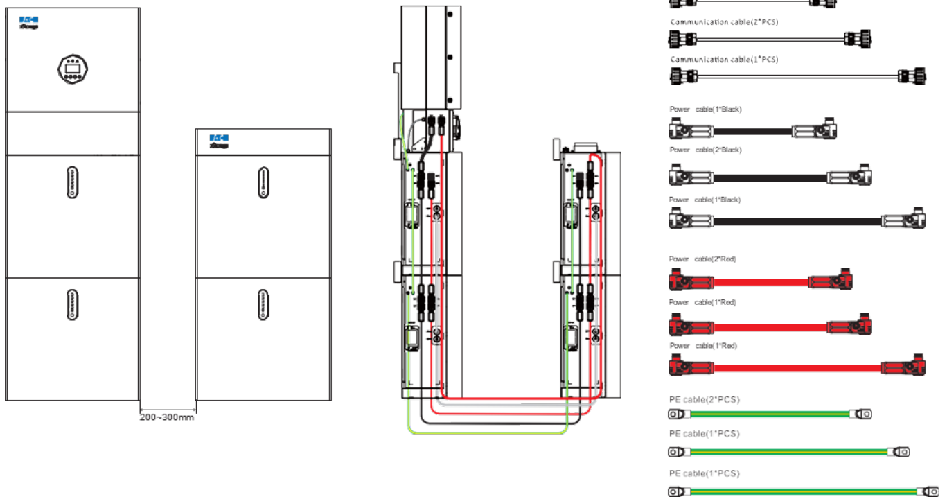
Figure 9. Accessory cables 4
