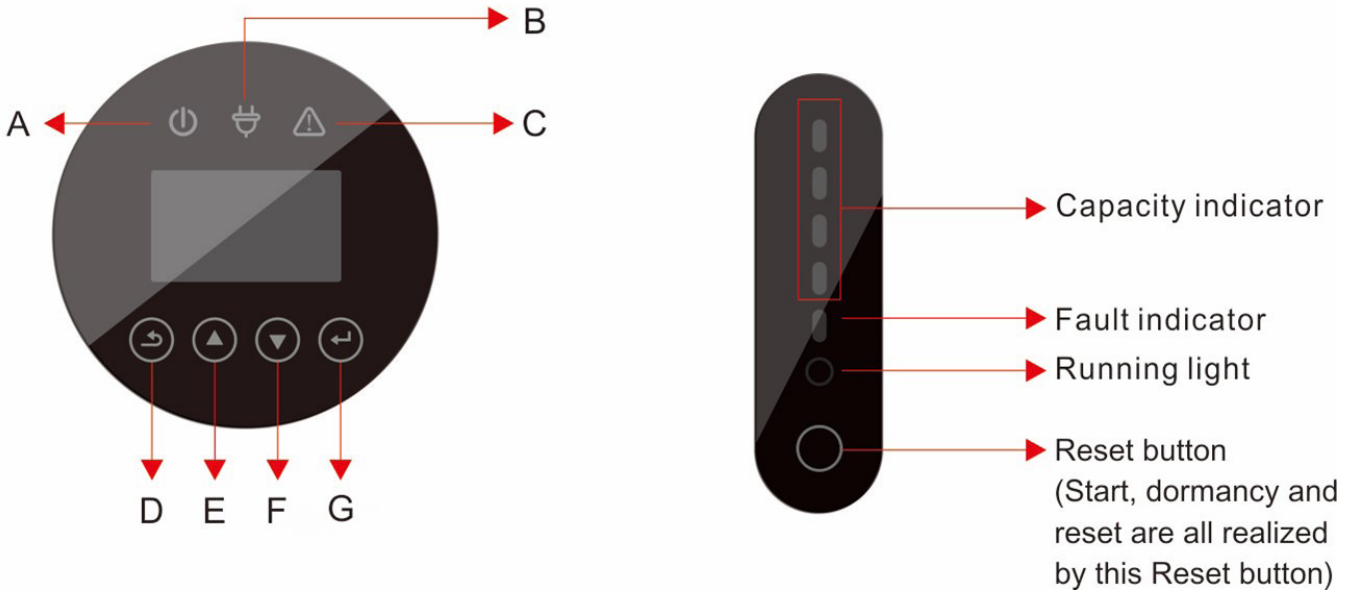
Figure 17. Hybrid Inverter EMS Interface and PACK interface
