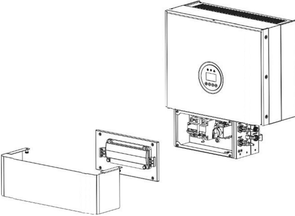
Figure 14. Cable Box Part without Covers - Front View
