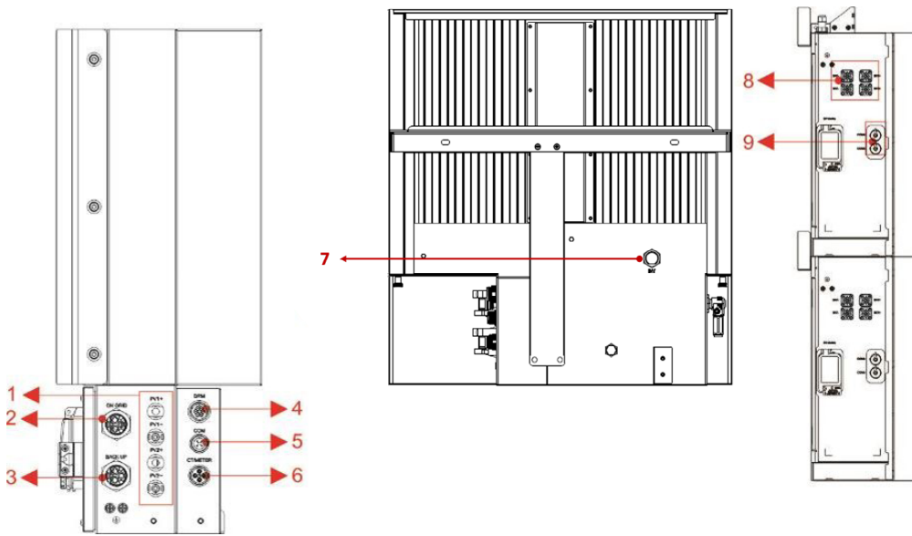
Figure 15. Cable Box Part without Covers
