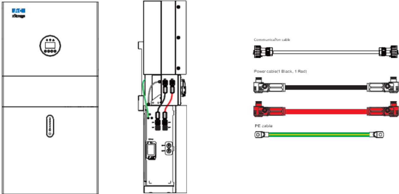
Figure 6. Accessory cables 1
