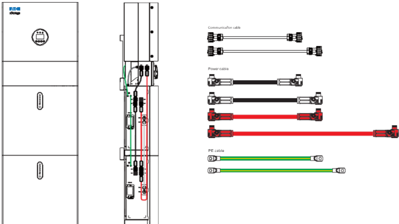
Figure 7. Accessory cables 2
