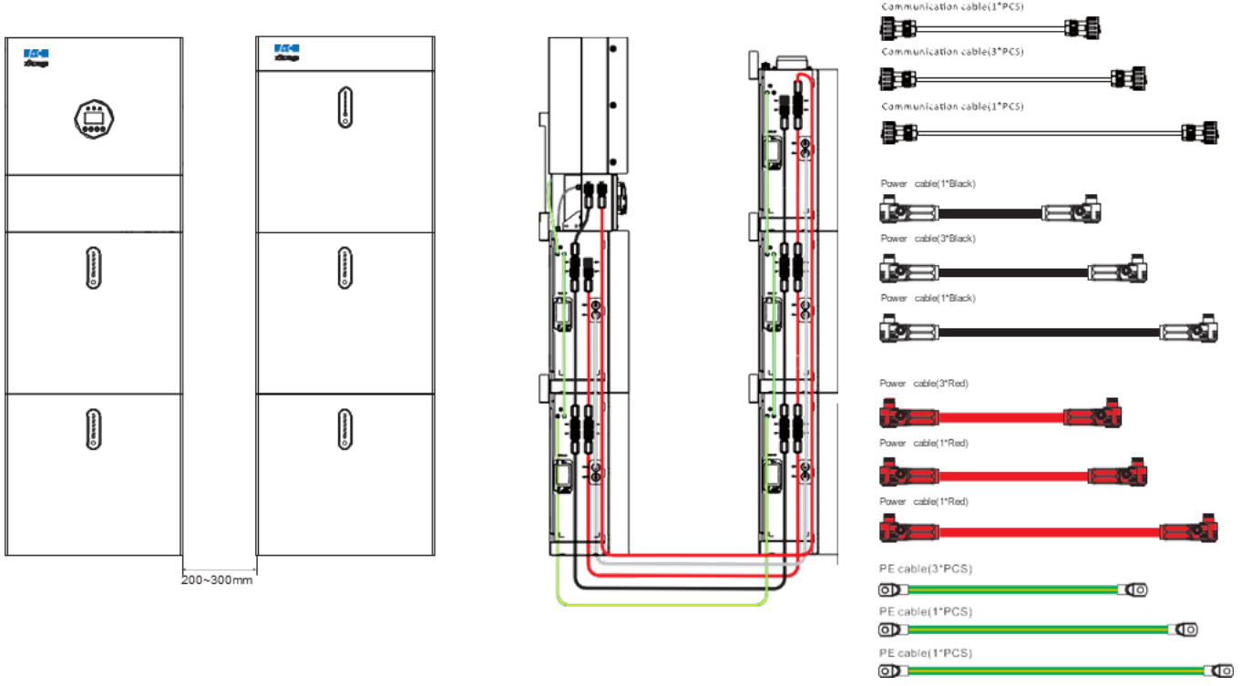
Figure 10. Accessory cables 5
