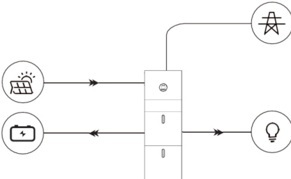
Figure 1. Self-consume operation mode
