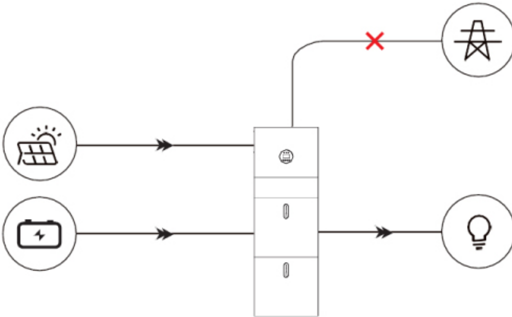
Figure 2. Battery priority operation mode
