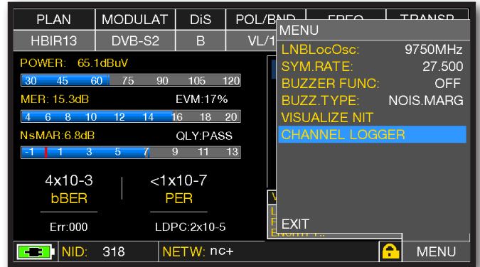
Touch "CHANNEL LOGGER".
