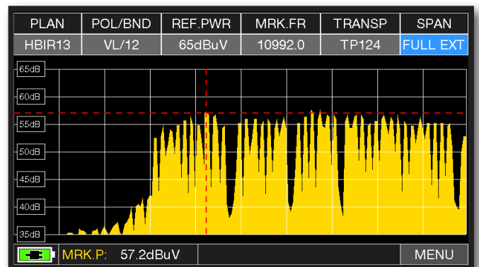
SAT spectrum SPAN "Full EXT" (from 230 to 2610 MHz).
