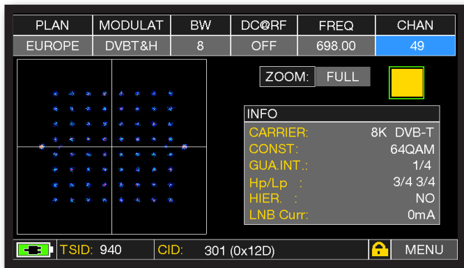
Constellation DVB-T.
