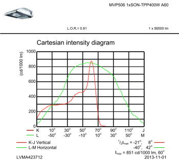
OFCC_MVP506 1xSON-TTP400W A60-Cartesian Outdoor (combined)
