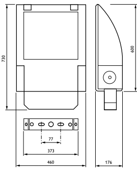
OptiFlood MVP506
