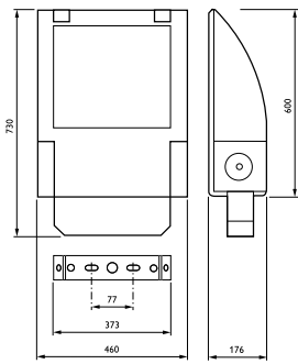
OptiFlood MVP506
