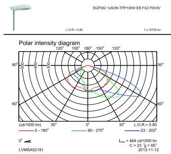
OFPC1_SGP352 1xSON-TPP100W EB FX2 P3H3V.EPS
