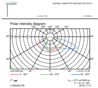
OFPC1_SGP352 1xSON-TPP100W EB FX2 P2H1V.EPS
