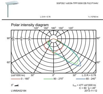
OFPC1_SGP352 1xSON-TPP100W EB FX2 P1H4V.EPS
