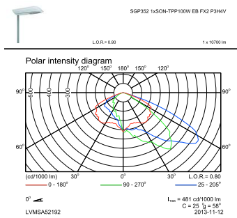
OFPC_SGP352 1xSON-TPP100W EB FX2 P3H4V-Polar Outdoor (combined)
