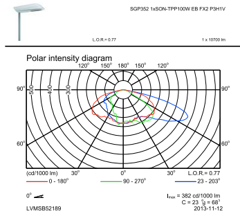
OFPC_SGP352 1xSON-TPP100W EB FX2 P3H1V-Polar Outdoor (combined)
