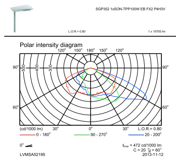
OFPC_SGP352 1xSON-TPP100W EB FX2 P4H3V-Polar Outdoor (combined)
