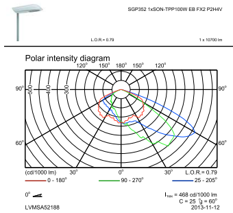
OFPC_SGP352 1xSON-TPP100W EB FX2 P2H4V-Polar Outdoor (combined)
