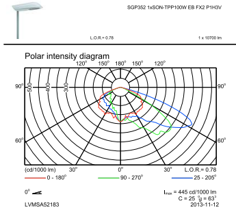
OFPC1_SGP352 1xSON-TPP100W EB FX2 P1H3V.EPS
