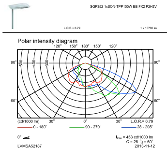
OFPC1_SGP352 1xSON-TPP100W EB FX2 P2H3V.EPS
