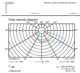
OFPC1_SGP352 1xSON-TPP100W EB FX2 P2H2V.EPS
