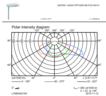
OFPC1_SGP352 1xSON-TPP100W EB FX2 P4H1V.EPS
