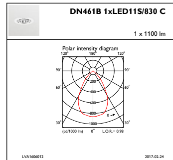
IFPC1_DN461B1xLED11S830C
