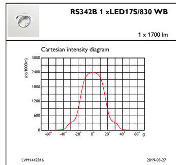
IFCC1_RS342B1xLED175S830WB
