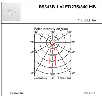
IFPC1_RS343B1xLED27S840MB
