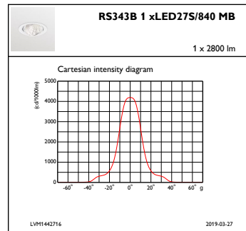
IFCC1_RS343B1xLED27S840MB
