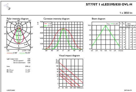
IFAS1_ST770T1xLED39S830OVL-H
