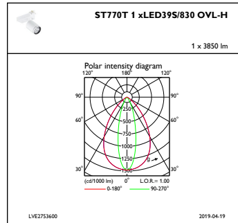
IFPC1_ST770T1xLED39S830OVL-H
