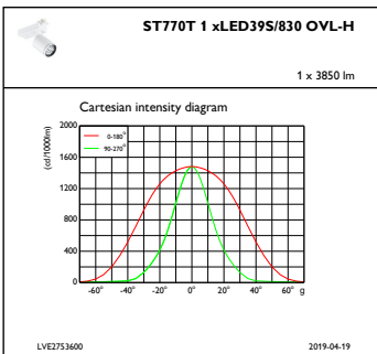
IFCC1_ST770T1xLED39S830OVL-H
