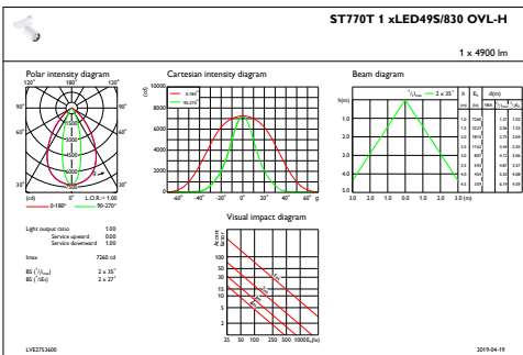
IFAS1_ST770T1xLED49S830OVL-H
