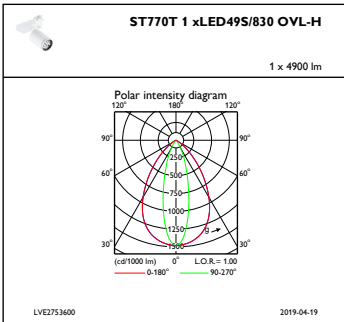
IFPC1_ST770T1xLED49S830OVL-H
