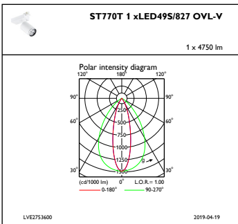
IFPC1_ST770T1xLED49S827OVL-V
