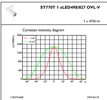
IFCC1_ST770T1xLED49S827OVL-V
