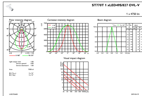
IFAS1_ST770T1xLED49S827OVL-V
