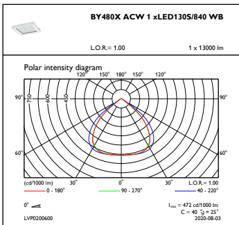
OFPC1_BY480XACW1xLED130S840WB
