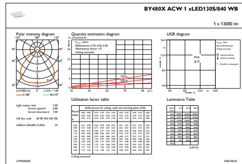
IFGU1_BY480XACW1xLED130S840WB
