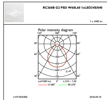
IFPC1_RC360BG2PSDW60L601xLED34S840
