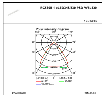
IFPC1_RC530B1xLED345830PSDW8L120
