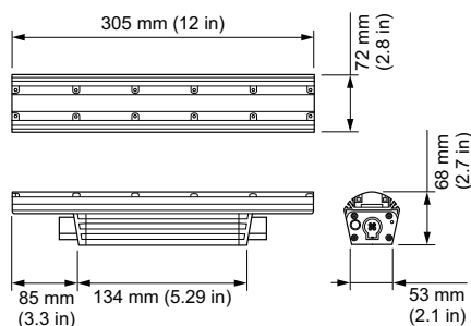
eW Graze MX Powercore
