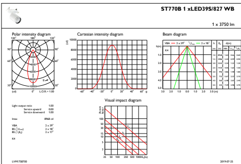
IFAS1_ST770B1xLED39S827WB
