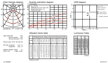
IFGU_DN570B PSE-E 1xLED20S/840 C--General uniform lighting
