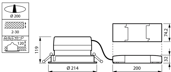
DN571B LED40S/840 DIA-VLC-E C WH
