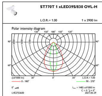
OFPC1_ST770T1xLED39S830OVL-H
