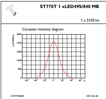
IFCC1_ST770T1xLED49S840MB
