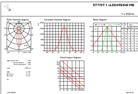
IFAS1_ST770T1xLED49S840MB
