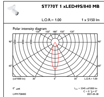
OFPC1_ST770T1xLED49S840MB
