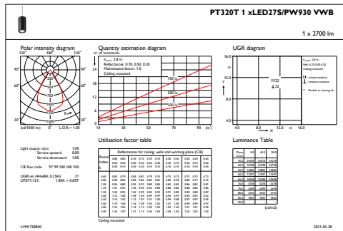
IFGU1_PT320T1xLED27SPW930VWB
