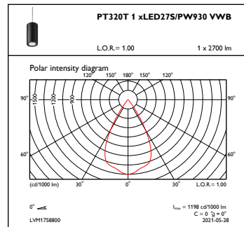
OFPC1_PT320T1xLED27SPW930VWB
