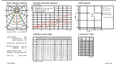
IFGU_4MX400 G3 491 1xLED55S/830 PSD NB-General uniform lighting
