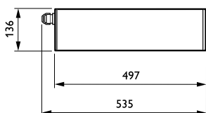
GearUnits ECB330/ECP330
