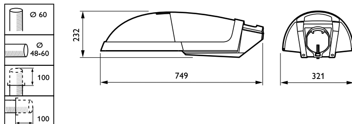
Selenium SGP340
