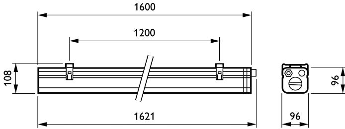
WT470C LED64S/840 PSU NB TC L1600
