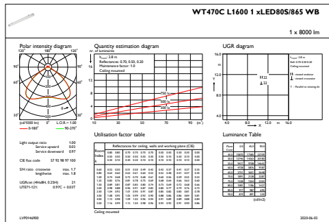
IFGU1_WT470CL16001xLED80S865WB
