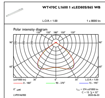
OFPC1_WT470CL16001xLED80S865WB
