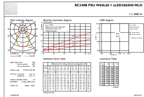
IFGU1_RC340BPSUW60L601xLED36S840MLO
