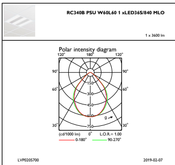
IFPC1_RC340BPSUW60L601xLED36S840MLO
