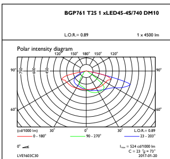
OFPC1_BGP761T251xLED45-4S740DM10
