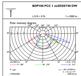
OFPC1_BDP100PCC1xLED50740DW
