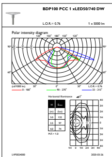
OFPL1_BDP100PCC1xLED50740DW
