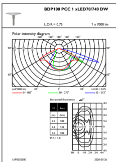
OFPL1_BDP100PCC1xLED70740DW
