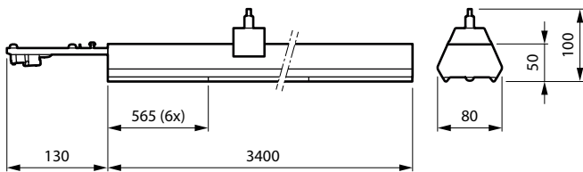
LL234X 160S/840 2x PSU WB 5x1.5
