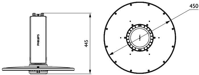
BY121P G4 LED200S/865 PSD WB
