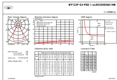
IFGU1_BY122PG4PSD1xLED250S865NB
