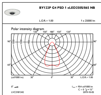
OFPC1_BY122PG4PSD1xLED250S865NB
