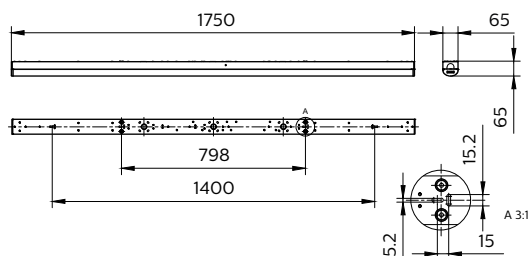
BN126C LED100S/840 PSU L1800
