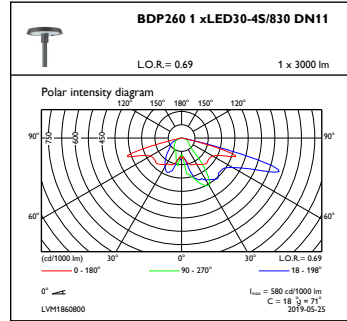
OFPC1_BDP2601xLED30-4S830DN11
