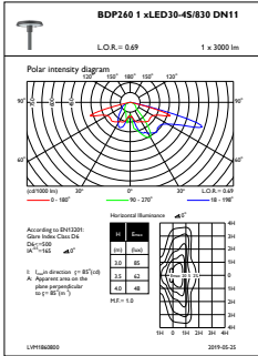
OFPL1_BDP2601xLED30-4S830DN11
