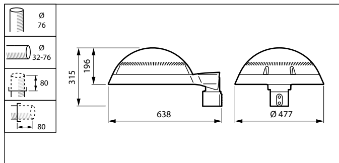
BDP268 LED94-4S/830 II DM10 48/60A
