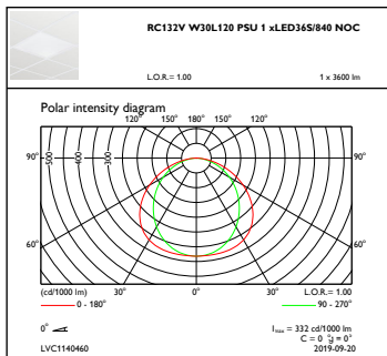
OFFPC1_RC132VW30L120PSU1xLED36S840NOC
