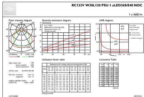
IFGU1_RC132VW30L120PSU1xLED36S840NOC
