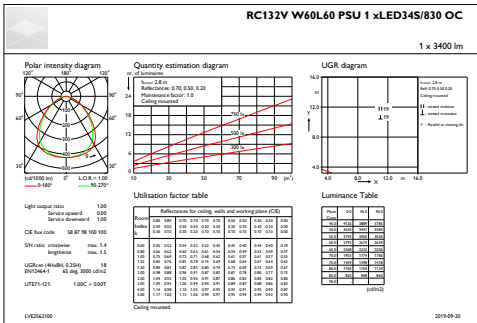
IFGU1_RC132VW60L60PSU1xLED34S830OC
