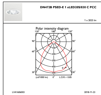
IFPC1_DN472BPSED-E1xLED20S830CPCC
