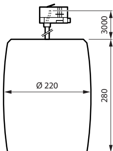
PT520T LED27S/840 PSU WB CURVE GR
