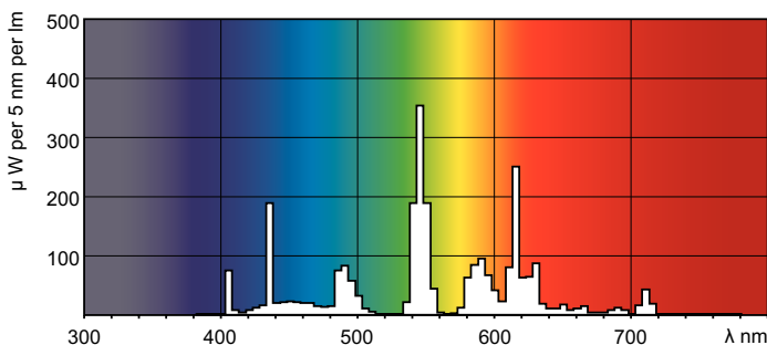
LDPO_TL-D8_835-Spectral power distribution Colour
