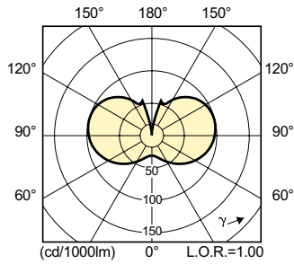
LDLD_CDO-ET_0004-Light distribution diagram
