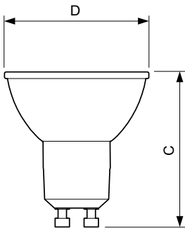
MASTER LED ExpertColor 3.9-35W GU10 940 36D
