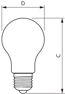
Bulb A67 100W 1521lm 4000K E27 ND Clear
