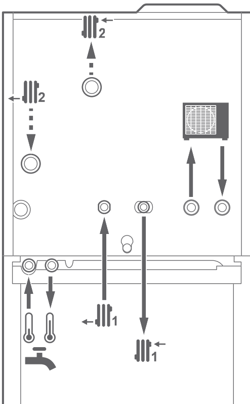
fig. 4 - Raccordements hydrauliques
